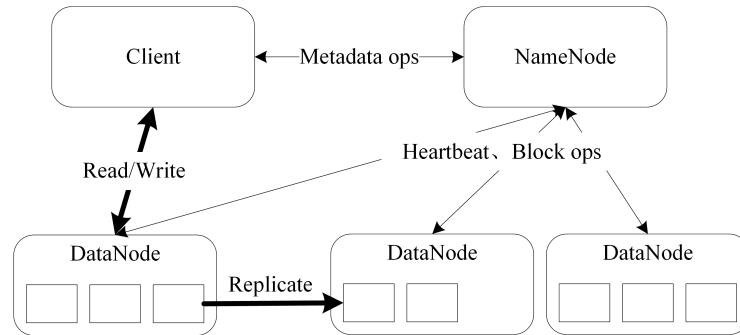
Fig. 1. HDFS Architecture
