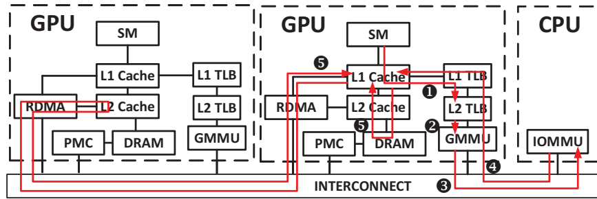
Fig. 2: Distributed address translation architecture
