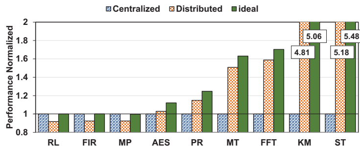
Fig. 3: Comparison of different address translation architecture
