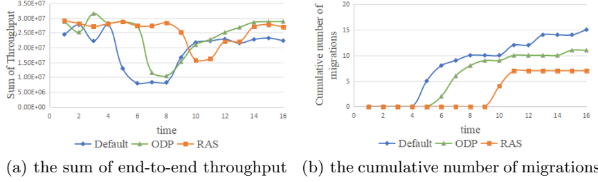
Fig. 3. Operator instance allocation analysis.
