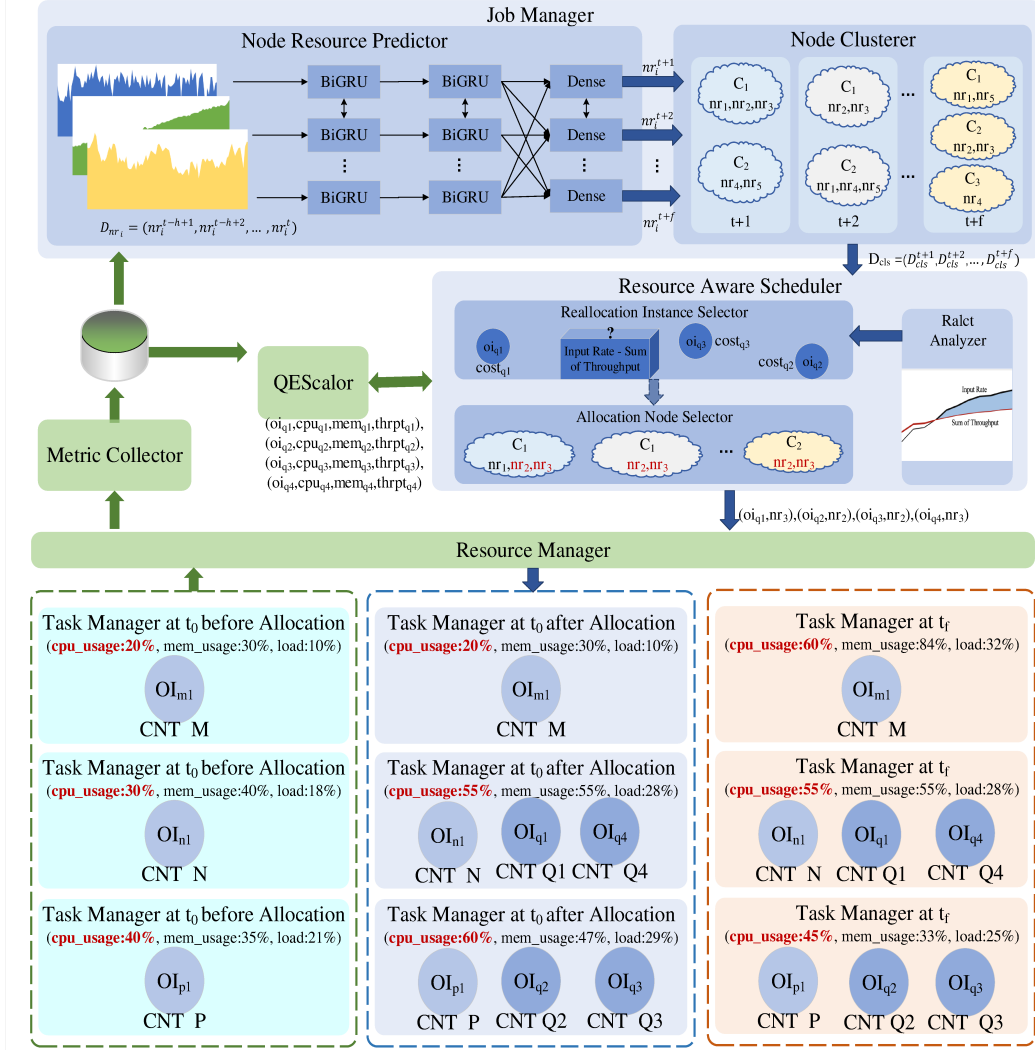
Fig. 1. DROAllocator architecture.
