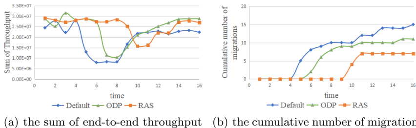
Fig. 3. Operator instance allocation analysis.
