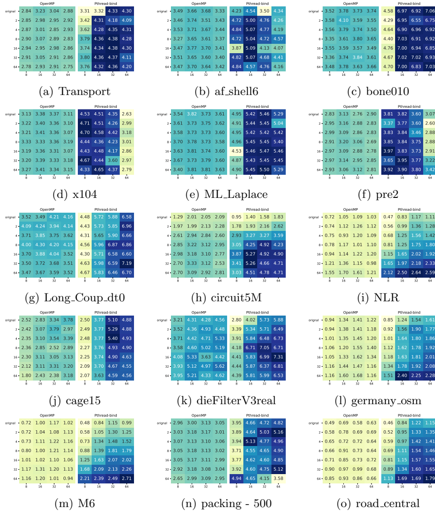
Fig. 5. Performance of OpenMP SpMV (left) and NUMA-Aware SpMV (right) on Phytium 2000+. In each subfigure, x-axis and y-axis refer to the number of threads and partitions, respectively. The heatmap values are in single precision GFlop/s.
