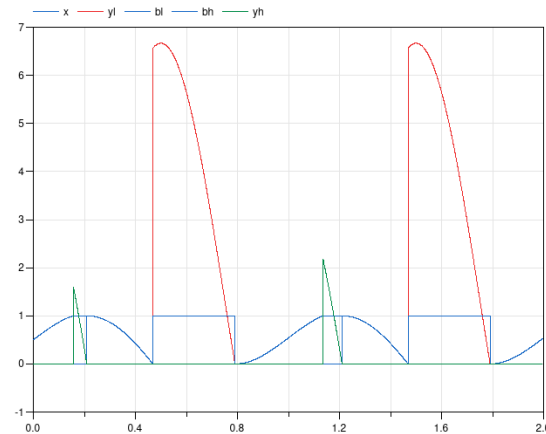
Figure 30. Simulation of the Water Tank system in RIMIS form with Dymola 2021.
