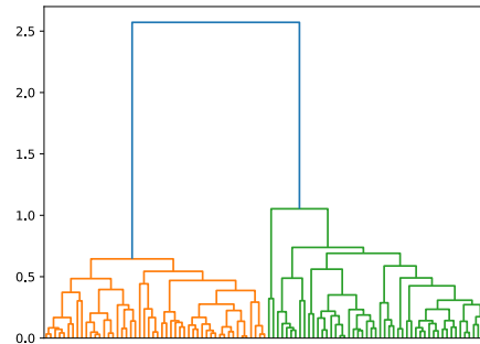
Figure 6.3: Toy experiment of a hierarchical clustering experiment. The data is sampled from two von Mises-Fisher distributions (left). A dendrogram is computed from the distance matrix (right).
