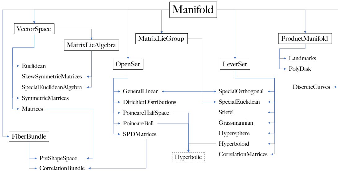
Figure 2.9: Architecture of the manifolds of geomstats . The abstract base classes are in black bounded boxes. Inheritance is shown by blue arrows. Hyperbolic is an exception as it is a common interface to the different representations of hyperbolic geometry.
