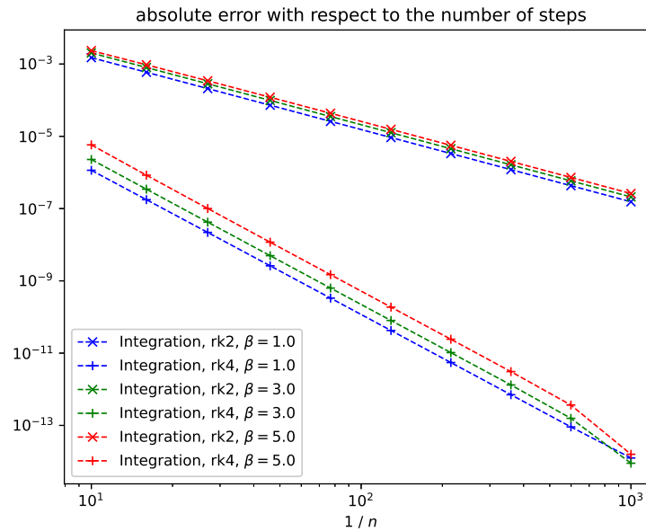
Figure 4.4: Norm of the absolute error represented with respect to the number of steps.
