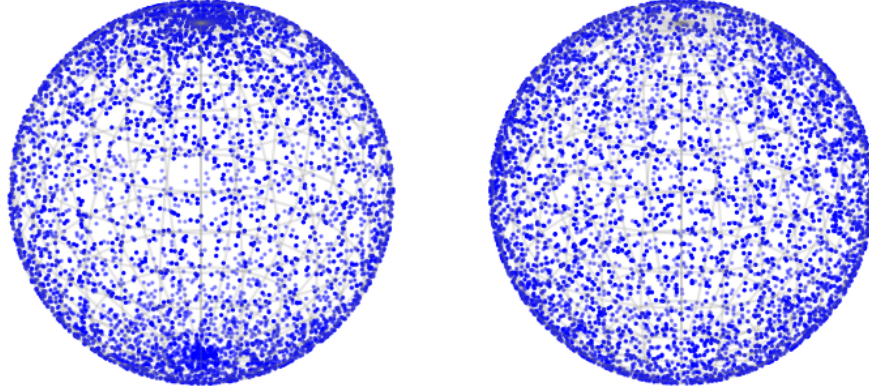
Figure 6.2: Comparison of the naive sampling from a uniform distribution on the spherical coordinates (left) and a more appropriate scheme that respects the isotropy of the sphere (right). In the naive case, points accumulate near the poles and are sparser around the equator.
