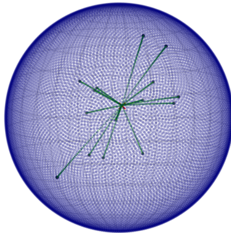
Figure 6.4: Fréchet mean on the sphere
