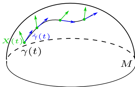
Figure 3.1: Representation of a parallel vector field X (green) along a curve \gamma (blue). The orientation of X with respect to the speed \dot{\gamma} of \gamma stays the same.
