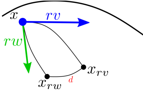
Figure 3.2: Drawing of the distortion of geodesics compared to Euclidean tangent vectors. Arrows represent tangent vectors, thin black lines represent geodesics and we use the notation x_v = \text{Exp}_x(v) . Curvature modifies the geodesic distance d compared with the distance between rv and rw in T_x M (adapted from Paulin, 2014, Section 3.6.3).
