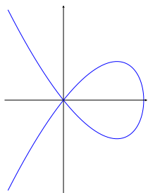
Figure 2.3: Nodal cubic M_1
