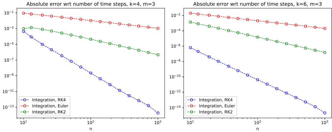
Figure 5.1: Convergence speed of the integration of Equation (5.9) for two orthonormal initial vectors v and \dot{\gamma}(0) , with respect to the number of steps. The curve \gamma is a horizontal geodesic here.
