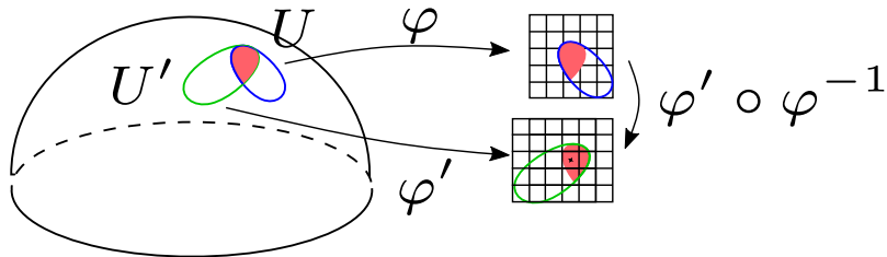
Figure 2.2: Transition maps.
