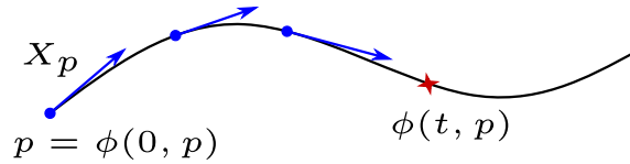
Figure 2.8: Example of a flow. The point \phi(t, p) is reached at time t by the integral curve of the vector field X .
