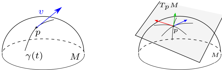
Figure 2.6: Left: Definition of a tangent vector as the derivative of a curve. Right: The collection of all tangent vectors forms a vector space.
