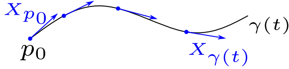
Figure 2.7: Example of an integral curve. The curve \gamma is obtained by integrating the vector field X (blue), meaning that X_{\gamma(t)} is tangent to \gamma at all times.
