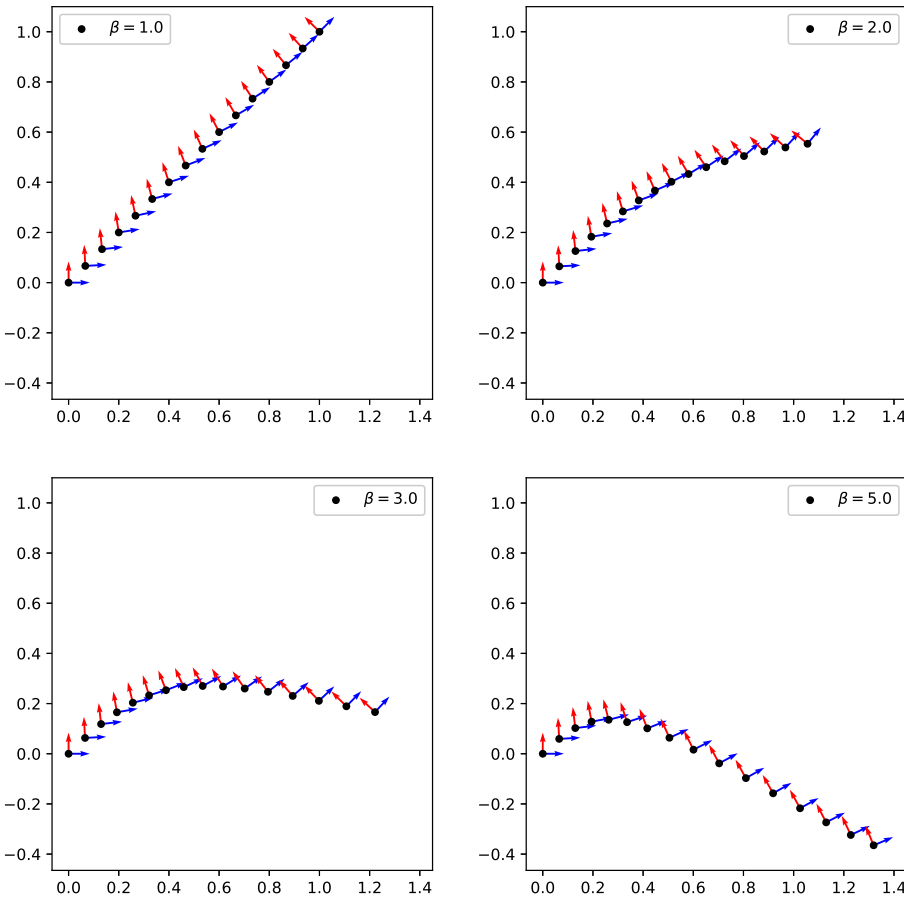
Figure 4.3: Visualization of geodesics on SE(2) with the same initial conditions and different values of \beta .
