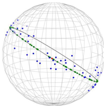
Figure 6.6: Example of geodesic regression on the sphere. The target data are the blue dots, the fitted values are in green, the regression geodesic in black, and the intercept ( \gamma ) in red.
