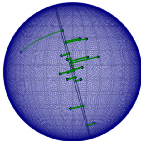
Figure 6.5: Example of PGA on the sphere. The target data are the black dots, the geodesics that realize the projection of each sample point to the principal geodesic are shown in green, the first geodesic subspace or principal geodesic is in gray, and the mean in red.
