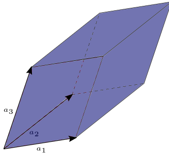
Figure 6.1: Volume spanned by three vectors in \mathbb{R}^3 .
