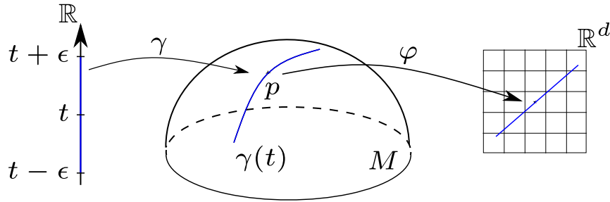
Figure 2.5: Definition of a smooth curve on a manifold.
