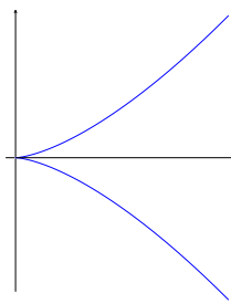
Figure 2.4: Cuspidal curve M_2
