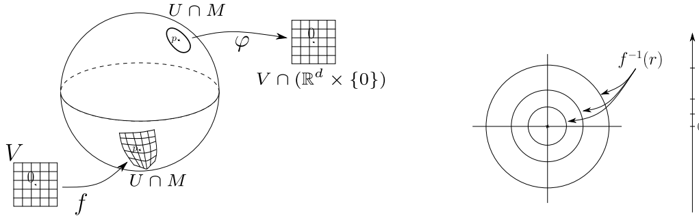
Figure 2.1: Left: Representation of a manifold, definition with local \varphi or by a local immersion f . Right: Representation of a manifold defined by a submersion, in this case the distance to the origin.
