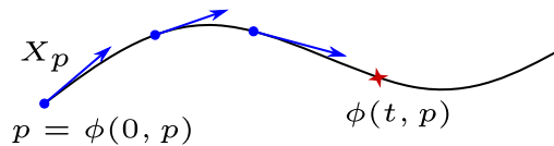
Figure 8: Example of a flow. The point \phi(t, p) is reached at time t by the integral curve of the vector field X .
