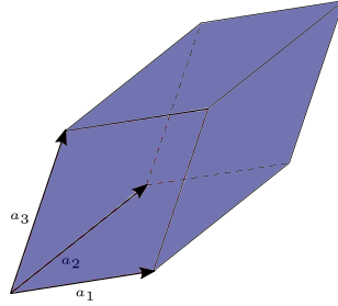
Figure 17: Volume spanned by three vectors in \mathbb{R}^3 .
