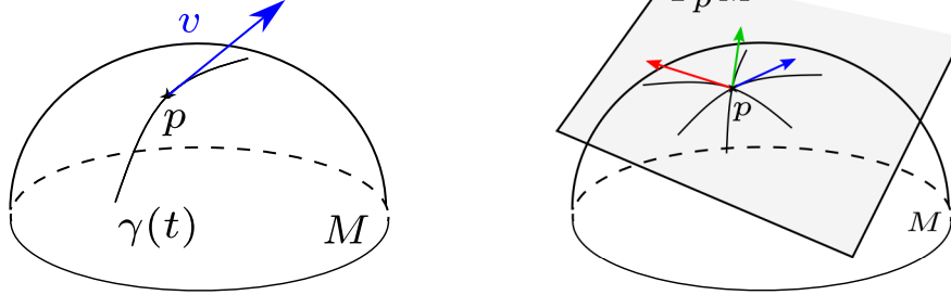
(a) Definition of a tangent vector as the derivative of a curve. (b) The collection of all tangent vectors forms a vector space.
