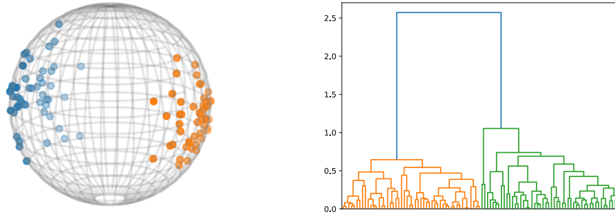
Figure 6.3: Toy experiment of a hierarchical clustering experiment. The data is sampled from two von Mises-Fisher distributions (left). A dendrogram is computed from the distance matrix (right).
