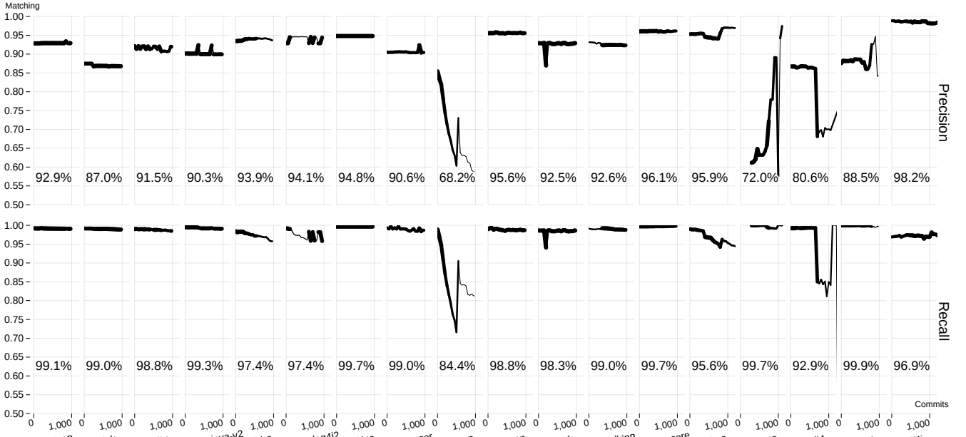
Figure 7: Validity of finding references with precision (top) and recall (bottom) per commit, with respective average.
