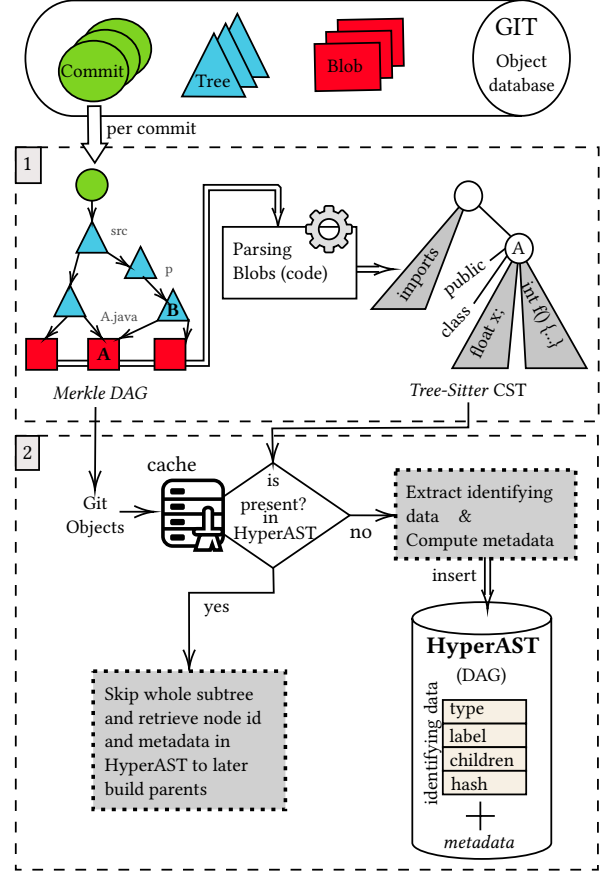
Figure 3: Overall approach of the HyperAST .
