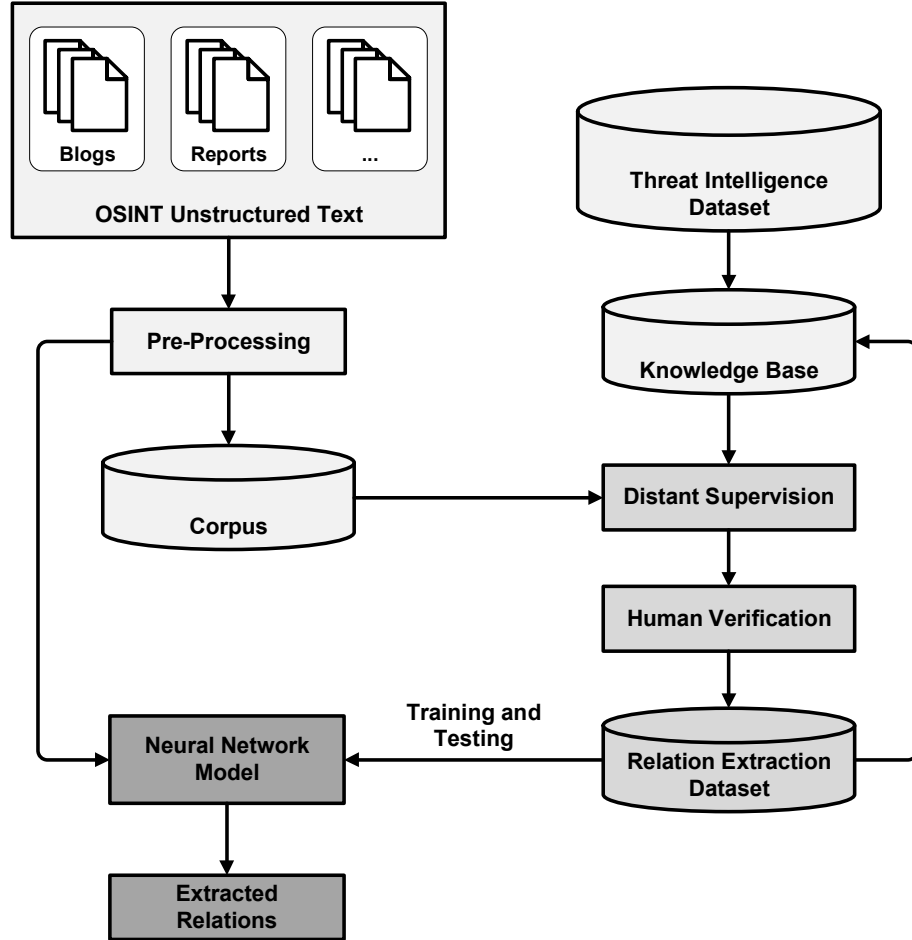
Figure 1. Framework workflow.
