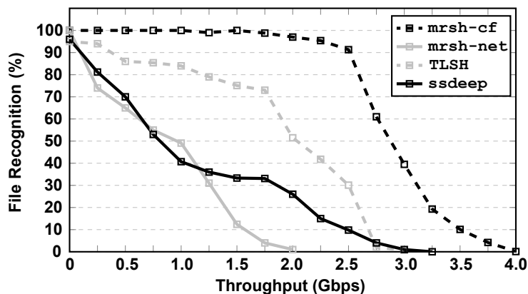
Figure 1. Initial throughput evaluations using the t5-corporus .
