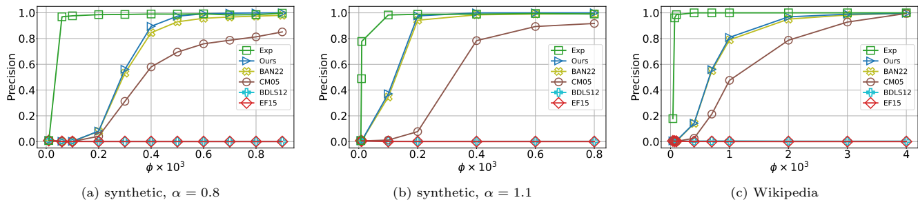
Figure 4: Precision as a function of the threshold \phi . (a) and (b) Synthetic traces: N = 1,000,000 , t = 5,000,000 , w = 10,000 , d = 8 , trials = 100. (c) Wikipedia trace: N = 292,332 , t = 1,000,000 , w = 5000 , d = 5 .
