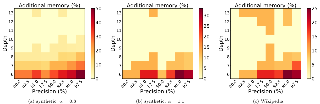
Figure 6: Additional memory required in comparison to the optimal setting for different depth values and precision targets (our model's estimations). (a) and (b) Synthetic traces: N = 1,000,000 , \phi = 5 \cdot 10^{-4} . (c) Wikipedia trace: 1 million requests, \phi = 10^{-3} .
