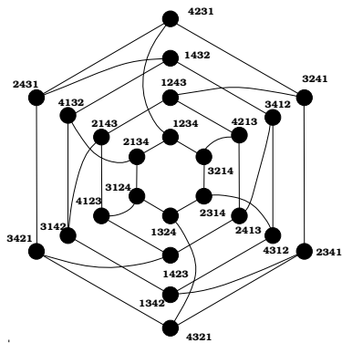
Fig. 2. Star-graph S(4)
