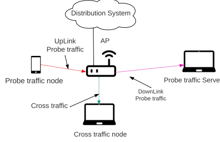
Figure 3: Aggregated cross traffic scenario. The probe traffic node and server estimate the current load. The cross traffic represents the current load of the system.
