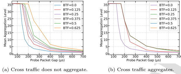
Figure 11: Simulated Mean Aggregation levels depending on cross traffic aggregation.
