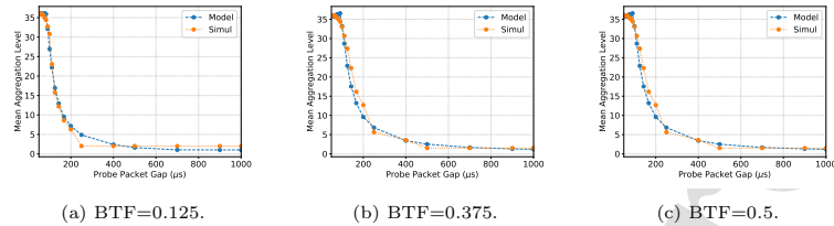
Figure 10: Mean agg levels, agg cross traffic, model vs NS-3 - 802.11ax traffic.
