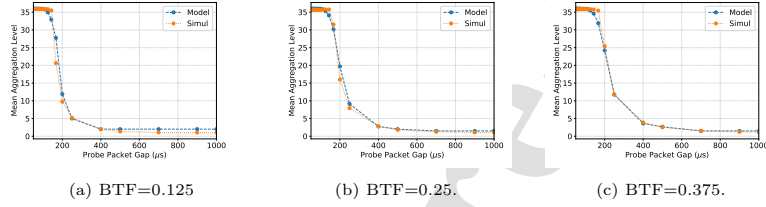
Figure 9: Mean agg levels, agg cross traffic, model vs NS-3 - Exp On/Off cross traffic.
