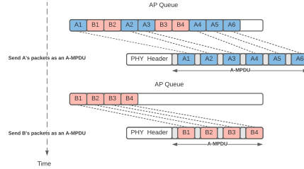
Figure 2: An Example of scheduling under frame aggregation.
