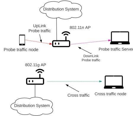
Figure 5: Scenario modeled by the model based on non-aggregated cross traffic.
