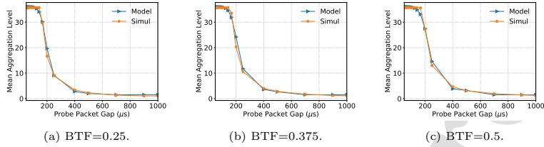
Figure 7: Mean aggregation levels, aggregated cross traffic, model versus NS-3 - MCS 15.
