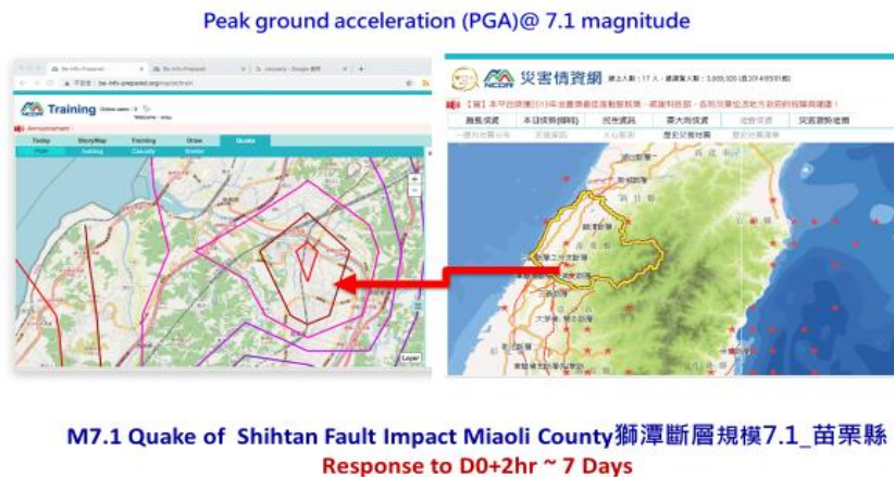
Fig. 5. A large-scale Earthquake Scenario, Source: NCDR
