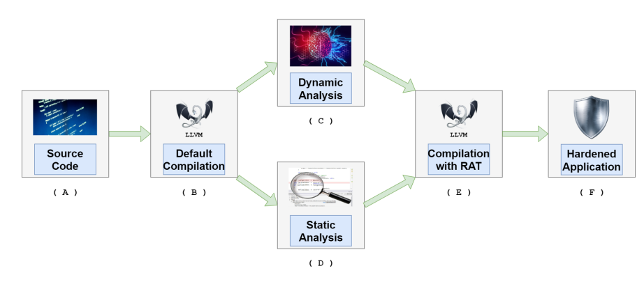
Fig. 1: Main steps of proposed register allocation technique (RAT).
