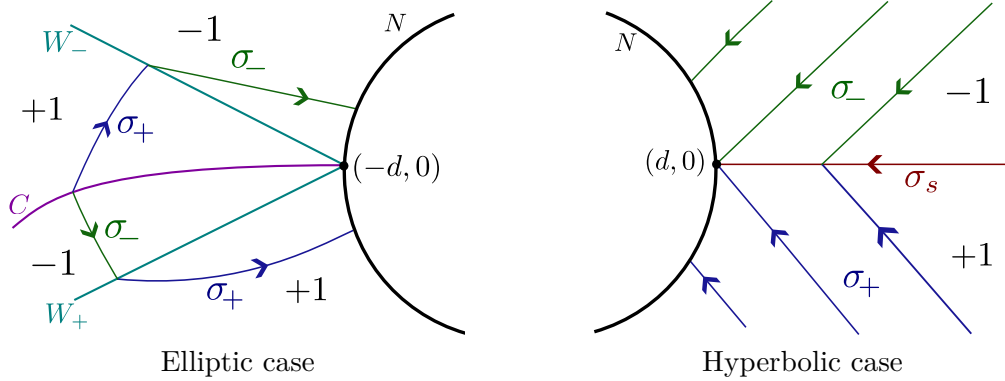
Figure 10. 2d-syntheses.
