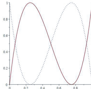
Figure 1: The cubic map C (solid line) and its mirror CM (points)
