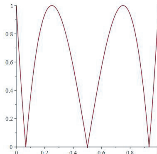
Figure 2: The dynamical system C \text{ xor } CM
