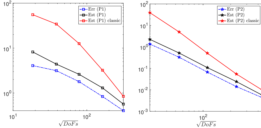
FIG. 8. Example 1. Convergence history of the error, error estimator of Equation 3.21 and the classical estimator for p = 1, 2 .
