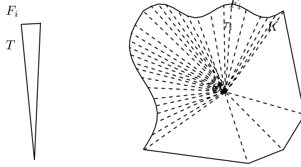
FIG. 5. Left: a triangle with one ‘small’ face. Right: a polytopic element with many ‘small’ faces.
