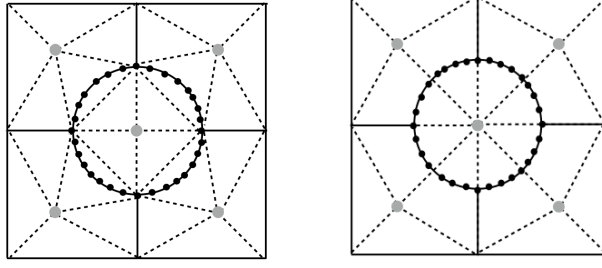
FIG. 3. A mesh with 5 elements (solid lines) and (dash lines). auxiliary constrained Delaunay mesh with 16 elements. The dual nodes belonging to the set \mathcal{P} of Definition 2.7 are marked with a grey bullet.
