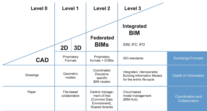
Fig. 1 Performance levels of BIM integration [7]
