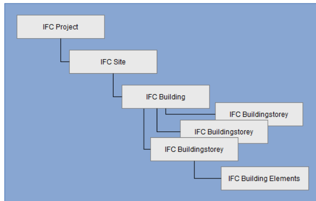
Fig. 2. IFC Tree-View [14]
