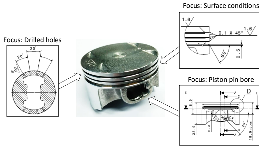
Fig. 7. Illustrative case study of cast aluminum piston
