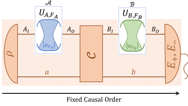
FIG. 2. A general circuit with FCO where \mathcal{A} is applied before \mathcal{B} . The target qubit and (possibly) some entangled “memory” system a are initially prepared in some state \rho . The target system then undergoes operation \mathcal{A} , after which the target and memory systems evolve through some channel \mathcal{C} . Operation \mathcal{B} is then applied to the target system, and a measurement is finally performed on the target and new memory system b , described by a POVM (E_+, E_-) . In our unitary discrimination task, the result of this POVM is taken as a guess for whether U_A and U_B (the unitaries that the operations \mathcal{A} and \mathcal{B} implement or approximate) commute or anticommute.
