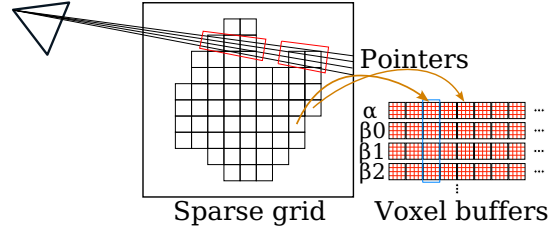
Figure 5. Sparse structure
