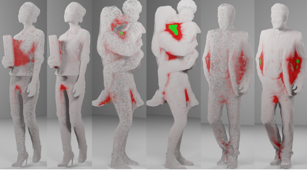
Figure 6. Chamfer heatmaps error comparison on synthetic human benchmark with 3 models, [13] vs ours.
