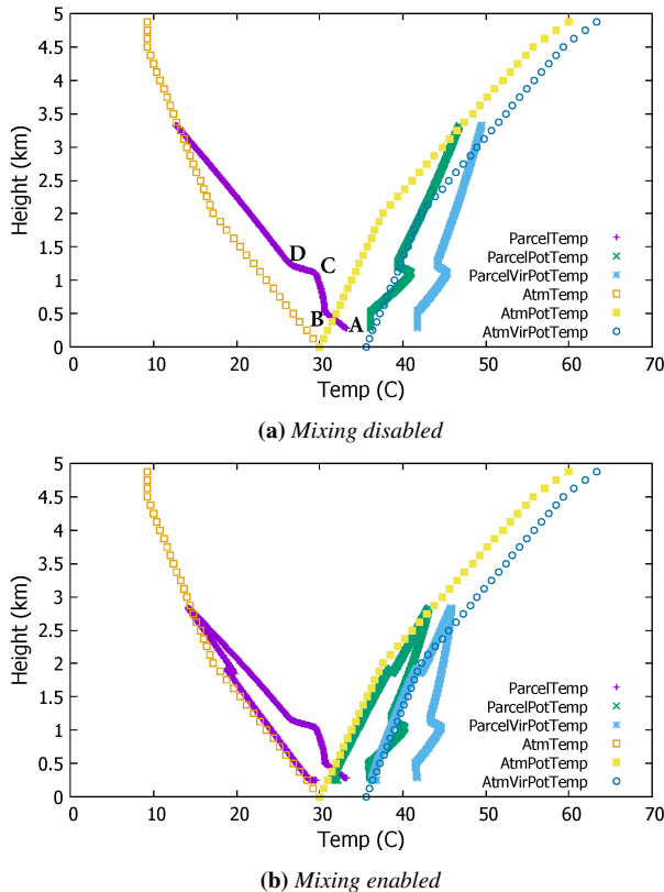
Figure 4: Parcel vs. environment temperatures ( T, \Theta, \Theta_v ) during single parcel simulation with (a) mixing disabled (b) mixing enabled.
