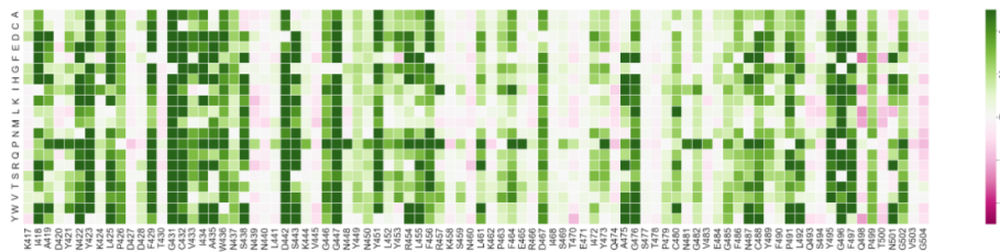
Fig. 2. Complete RBD-ACE2 interface mutagenesis heatmap where deep green color indicates positive FoldX force field \Delta energies (destabilising) and deep purple contrasting positive FoldX force field \Delta energies (stabilising).
