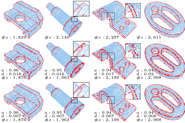
Figure 3. 3D models from the ABC dataset. Our method displaces the detected sharp feature points closer to the ground truth. Top row: ground truth. Middle row: detected raw sharp feature points. Bottom row: displaced sharp feature points. Sharp feature points are depicted in red, and smooth points are depicted in blue. a , d and \#s denote accuracy, point-to-feature distance and number of sharp feature points, respectively.
