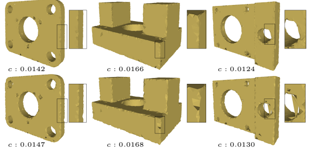
Figure 9. Reconstructed meshes using DSE meshing. First row: reconstruction from the consolidated 3D point clouds. Second row: reconstruction from the 3D input point clouds. c denotes the Chamfer distance between the reconstructed mesh and the ground truth mesh in the ABC dataset. DSE meshing is able to capture more details on sharp creases with consolidated point clouds and the Chamfer distance shows that the meshes are closer to ground truth compared to the original point clouds.
