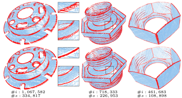
Figure 7. Scanned point clouds of Visionair repository. The first and the second rows show the detected predicted sharp feature points without and with displacement, respectively. \#i and \#s denote the number of input points and the number of detected sharp feature points, respectively.
