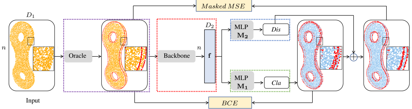
Figure 2. Overview of the proposed learning architecture. It comprises four modules: point-to-feature oracle (purple dash), point descriptor extractor (red dash), sharp feature detector (green dash) and displacement predictor (blue dash). Point-to-feature oracle module is only used for training. It introduces noise to the input, computes the ground truth classification labels and the ground truth displacement vectors. A backbone is used to extract high dimensional representations \mathbf{f} (size: n \times D_2 ) in the point descriptor extractor module. MLP stands for multi-layer perceptron. Cla and Dis represent binary sharp feature labels and displacement vectors, respectively. \oplus adds the corresponding predicted displacement vectors to detected sharp feature points to make them lie closer to the ground truth sharp features. BCE and Masked MSE are two losses calculated base on Cla , Dis and the ground truth generated by the oracle.
