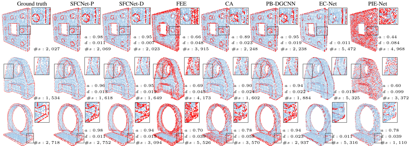
Figure 6. Visual comparisons with supervised and unsupervised methods on selected models from the test set. According to the closeups, our methods can detect more meaningful sharp feature points that are closed to the sharp features.
