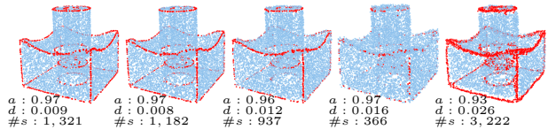
Figure 5. Visual comparison with different pairs of sharp distance thresholds and noise levels. From left to right, the pairs of sharp distance thresholds and noise levels have the same order as in Table 1. An incompatible choice of d_{\max} and n (the 4th model) leads to a bad result.
