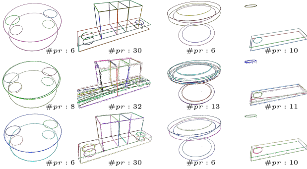
Figure 8. Feature line extraction results using RANSAC. From top to bottom: results of dense, uniformly sampled points on ground truth feature creases, results of the detected sharp feature points without displacement, results of the consolidated sharp feature points by our SFCNet-P model. #pr denotes the number of detected primitives. The ones without displacement detect many wrong primitives and there are more outliers (black points) left after the detection.
