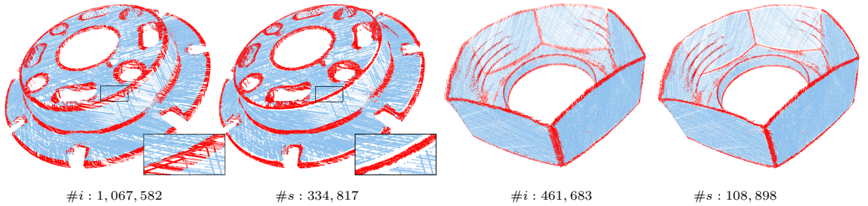
Figure 10: Scanned point clouds of Visionair repository. The first and the third image show the detected sharp feature points without displacement. The second and the forth ones show the predicted sharp feature points with displacement. \#i and \#s denote the number of input points and the number of detected sharp feature points, respectively.
