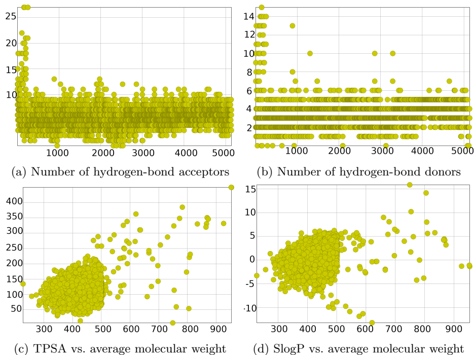
Fig. 2: Physicochemical properties of the set of selected 5141 compounds docked against target 3CLpro. Abbreviations used: TPSA – topological polar surface area; SlogP – logarithm of the enhanced atomic partition coefficient.
