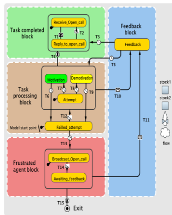
Fig. 2. Framework of a task.
