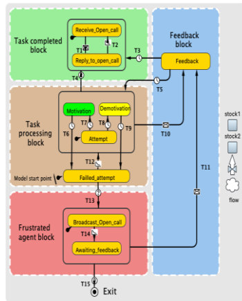
Fig. 2. Framework of a task.
