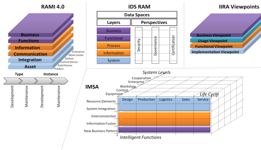
Fig. 1. RAMI 4.0, IIRA, IDS RAM and IMSA architecture approaches.
