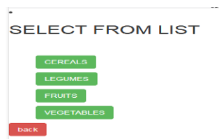
Fig. 7. Selection screen
