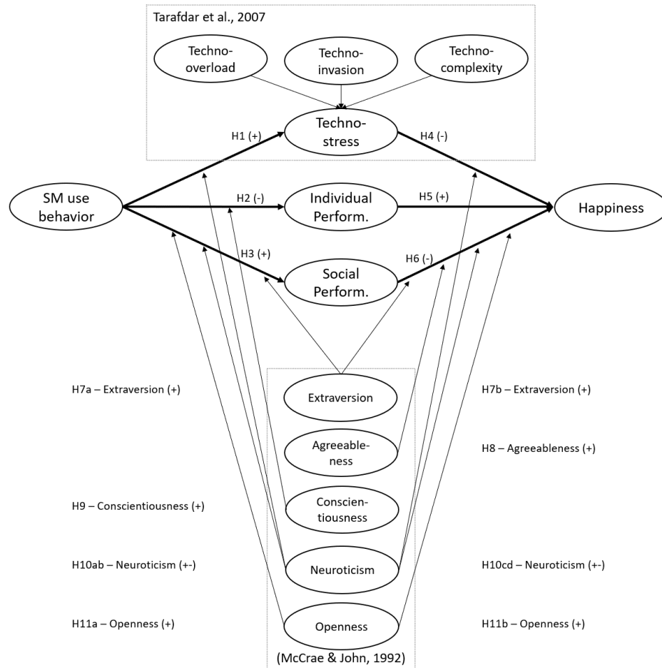
Fig. 1. Research model
