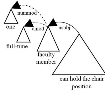
Fig. 3. Collapsed dependency tree representation of “One faculty member can hold the chair position.” R=\{\text{full-time,chair}\} second element here is captured using SRL tagger
