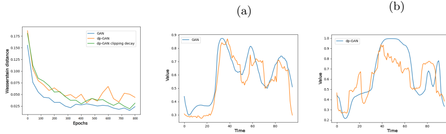
Fig. 2. Wasserstein distance
