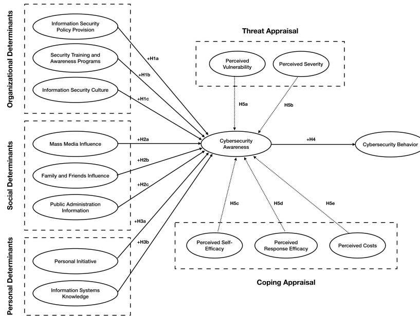
Fig. 1. Research Model
