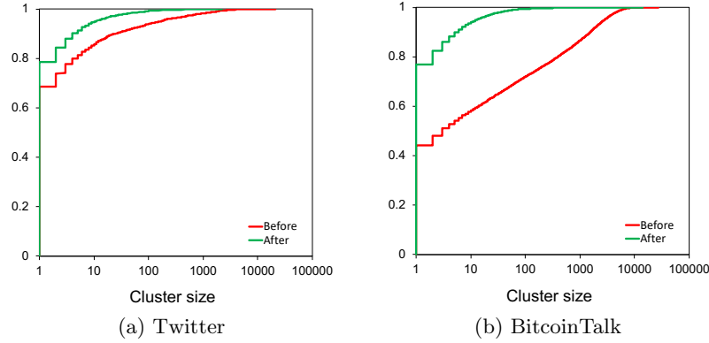
Fig. 2: CDFs of minimal clustering’s cluster size before and after trimming
