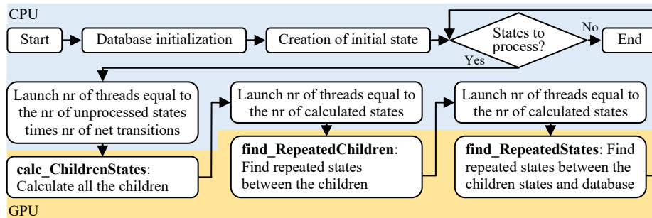
Fig. 1. Sequence of actions of the algorithm.
