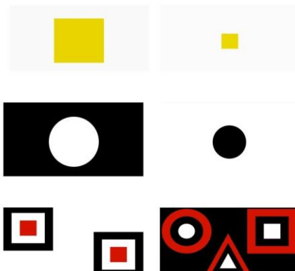
Fig. 2. Different characteristics of geometric figures
