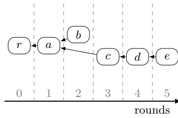
Fig. 2. Slots with parent relation in the tree model.
