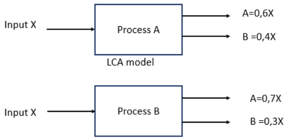
Figure 13 Differences in multi-output modelling between MFA and LCA
