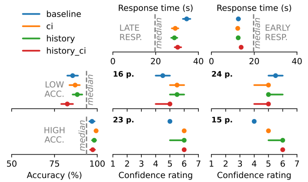
Fig. 9: Confidence ratings are broken down as per the participants' average compared to the median, for accuracy (rows) and response time (columns), with 95% confidence intervals for the median of confidence rating, and mean of accuracy and response time.
