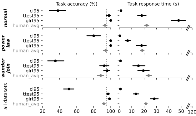
Fig. 8: Task accuracy and response time of automated decision procedures with 95% accuracy threshold (dotted line), for each dataset and overall, with 95% confidence intervals for mean values. In gray, the average human performance for reference.
