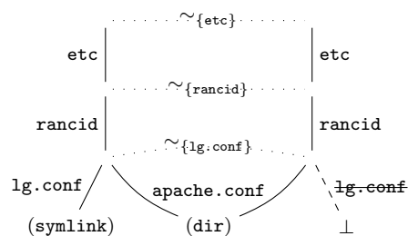
Fig. 4 Example of diagnosis: error case for preinst call in the package randid-cgi . This diagram displays knowledge about the initial file system (on the left side), and about the file system resulting from an attempt to execute the script (on the right). The respective roots of the two filesystem are on the top, downward edges represent links in the file system. A dotted edge describes a similarity relation, e.g. , the \sim_{\{randid\}} on the second dotted line means that the trees rooted at /etc coincide except possibly on the child named randid . \perp denotes the absence of a node. Finally, a leaf can be annotated by a property, e.g. , the annotation (dir) rooted at /etc/randid/apache.conf expresses that this node is a directory.
