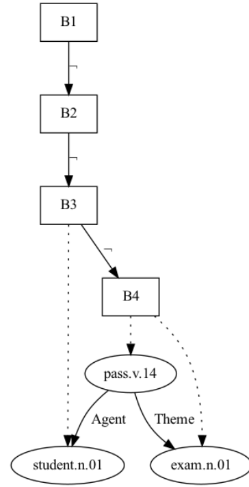
Figure 11: DRG for Not all the students passed the exam.
