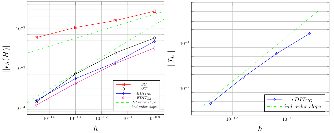
Figure 16: Hypersonic flow past a blunt body: grid-convergence analysis.
