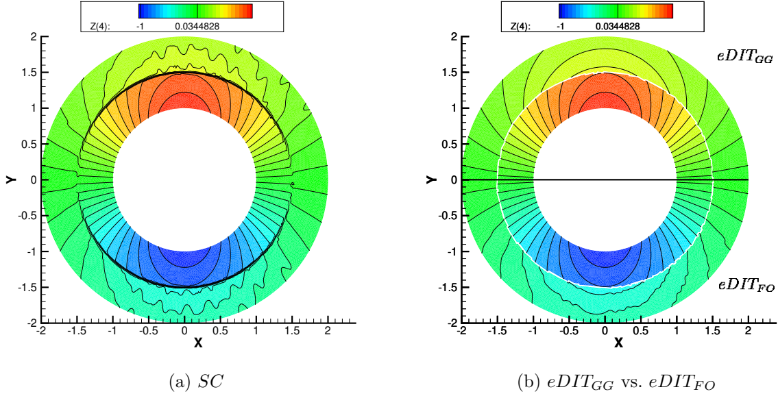
Figure 13: Transonic source flow: iso-contours comparison on grid level 2 w.r.t. Z_4 = \sqrt{pv} .
