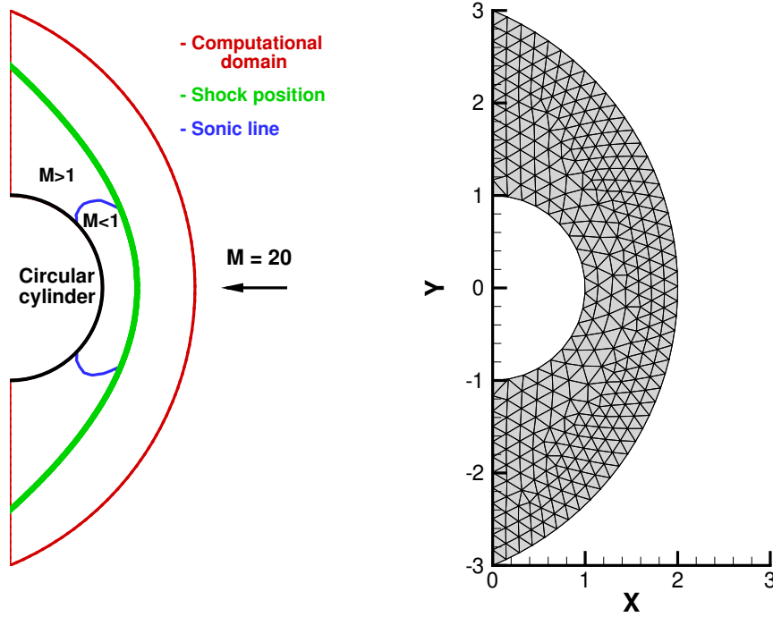
(a) Sketch of the computational domain. (b) Detail of the level 0 unstructured mesh.
