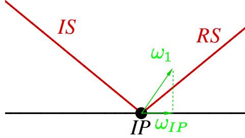
Figure 26: Supersonic channel flow: regular reflection at a solid wall and calculation of the displacement velocity of the point, IP, where the IS and RS meet.
