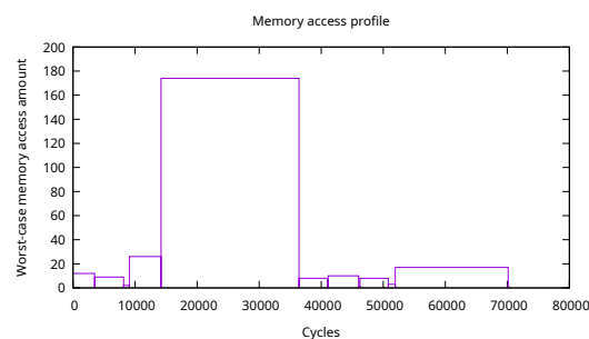
■ Figure 4 Example memory access profile ( minver , node-centric SESE regions, non-limiting large value of fuel parameter).
