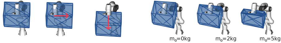
Fig. 2. Three images on the left show the shifting effect on the reachable space polytope \mathcal{P}_x produced by certain cartesian velocity at the beginning of the horizon, from left to right: \mathbf{x}_k = [0, 0, 0], [0, 1, 0] and [0, 0, -1] m/s. Three images on the right show the reducing effect on the polytope \mathcal{P}_x by three different carried object masses (left to right) m_o = 0, 2 and 5 kg. Horizon used is t_h=0.15 s and the robot is in initial configuration.
