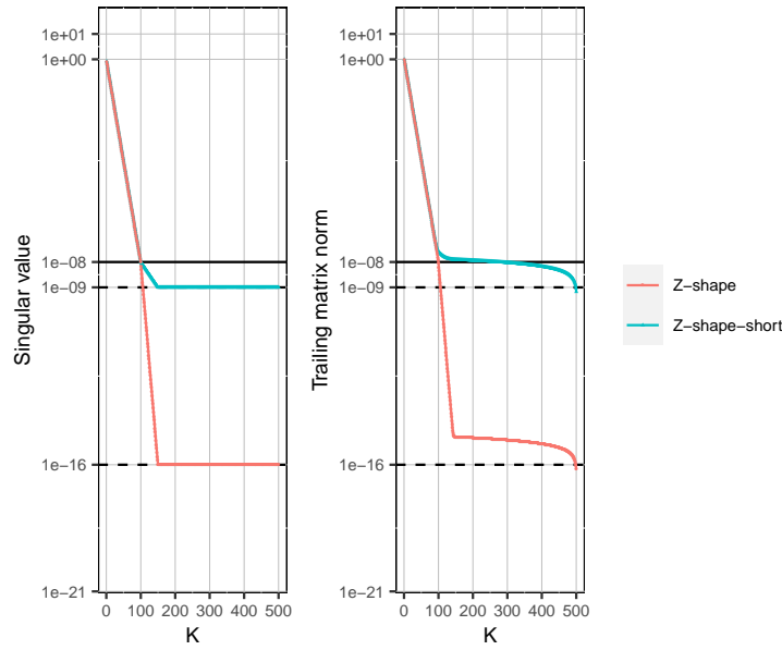
Figure 10: The Z-shape and Z-shape-short matrices of size 500 \times 500 , where the generation rank is r_G = \frac{20m}{100} = 100 at the generation precision \epsilon = 10^{-8} . The Frobenius norms of the trailing matrices at each index ( \frac{\|A_{22}^{(K)}\|_F}{\|A\|_F} ) are on the right, while the singular values at each index ( \sigma_K ) are on the left. The x-axis stands for the matrix indices. Both matrices have the same singular values up to the index r_G = 100 . However, after this point, Z-shape case singular values decrease faster and reach to almost machine precision at the index \frac{3}{4}r_G , whereas the Z-shape-short case singular values reach to \frac{\epsilon}{10} = 10^{-9} at this index.
